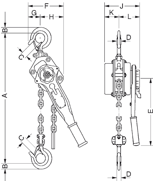
Model Silverline HZS 500 - 2000 kg, single fall
